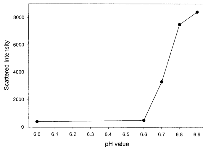
FIGURE 3 pH dependence of total scattered intensity of a 0.5 mg/ml CA protein solution, measured at 90° scattering angle.
