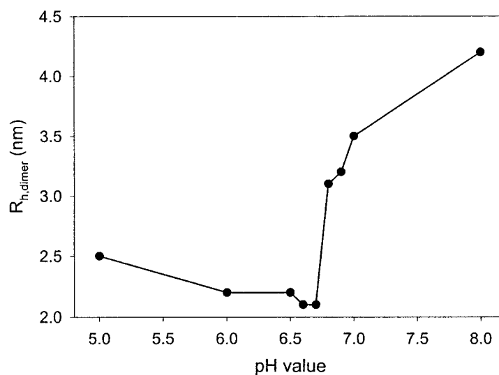
FIGURE 5 Apparent hydrodynamic radius ( R_h ) of CA dimers at different pH values, measured by DLS at 90° scattering angle.
